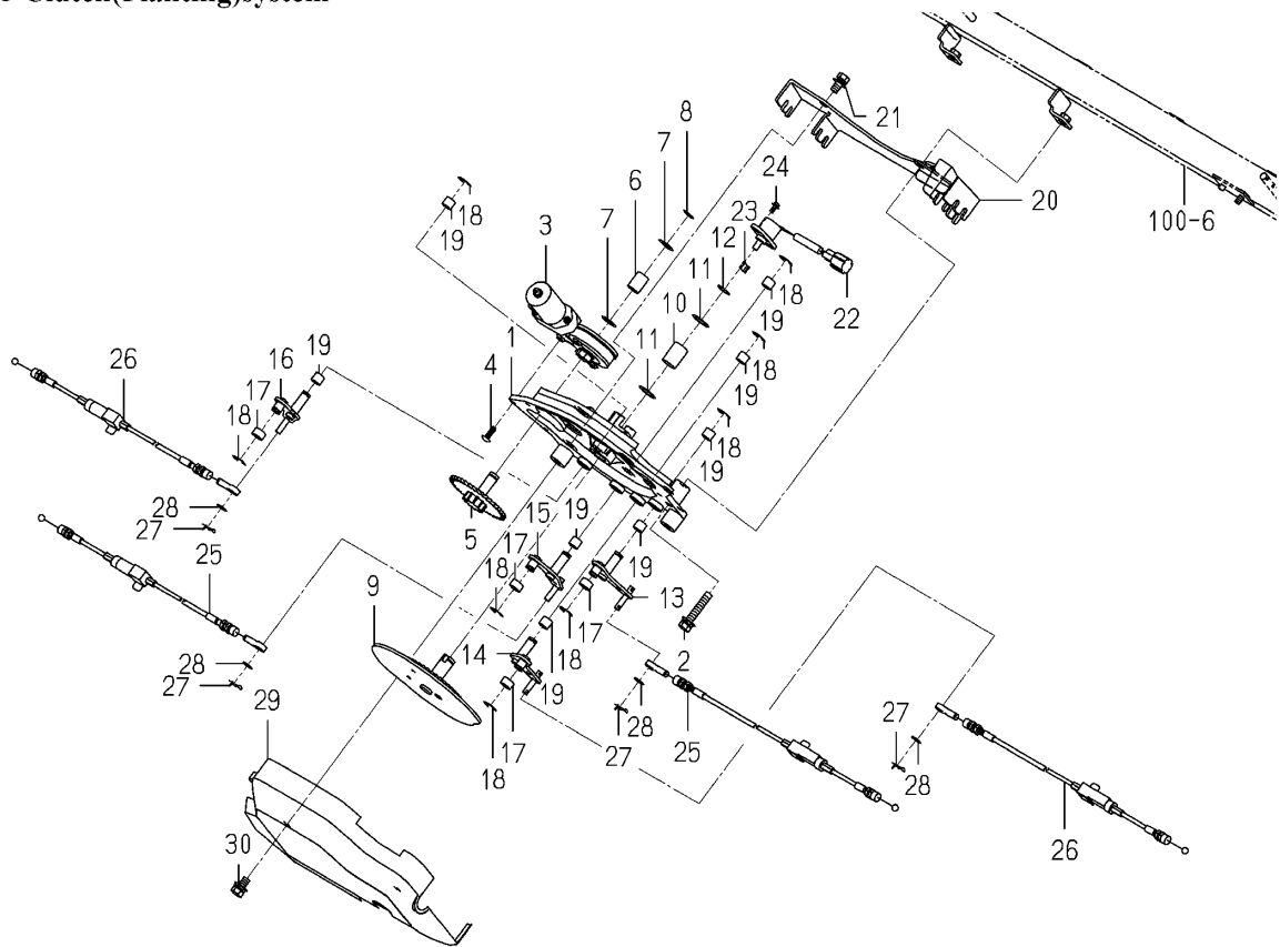
Fig.073 Clutch(Planting)system
