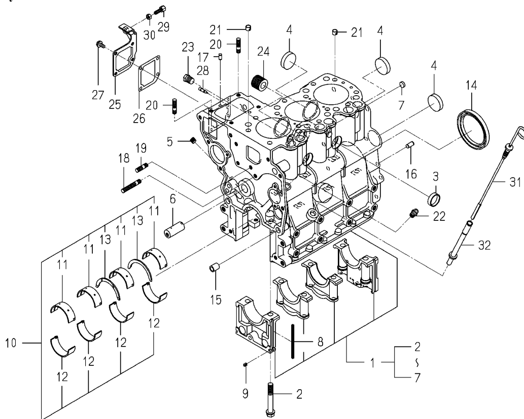
Fig.005 Cylinder Block
