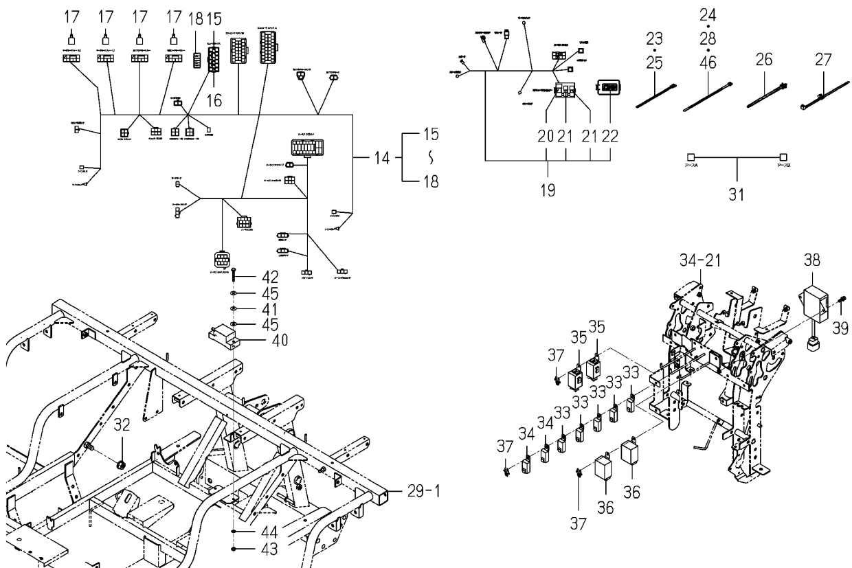
Fig.067a Harness(Traveling Section)system(2/2)
