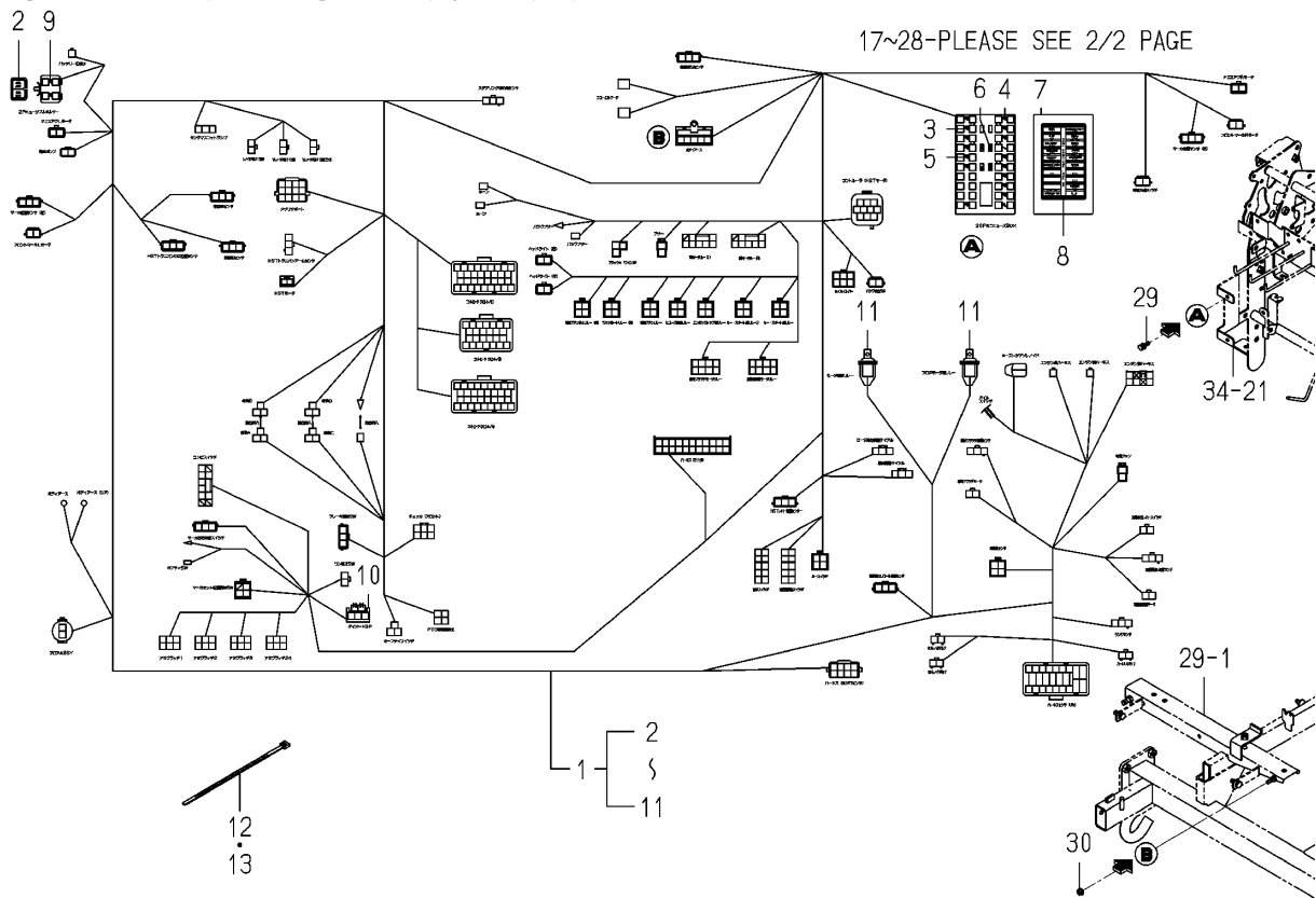
Fig.067 Harness(TrAVELING SECTION)system(1/2)
