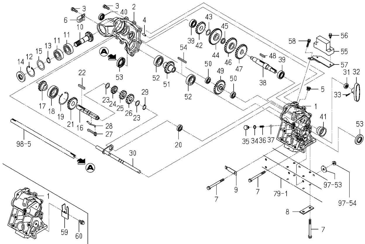
Fig.081 Slide System
