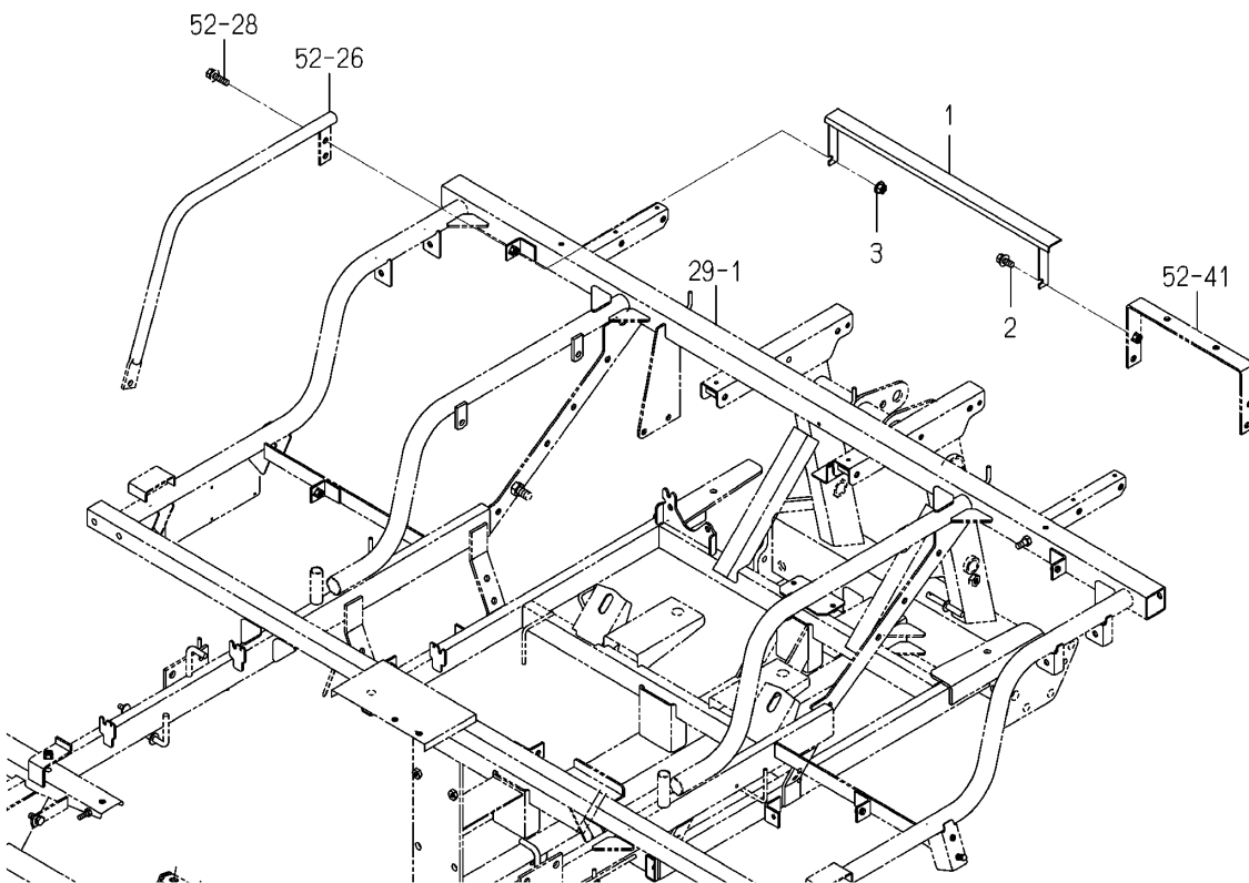
Fig.053 Step(Main)system
