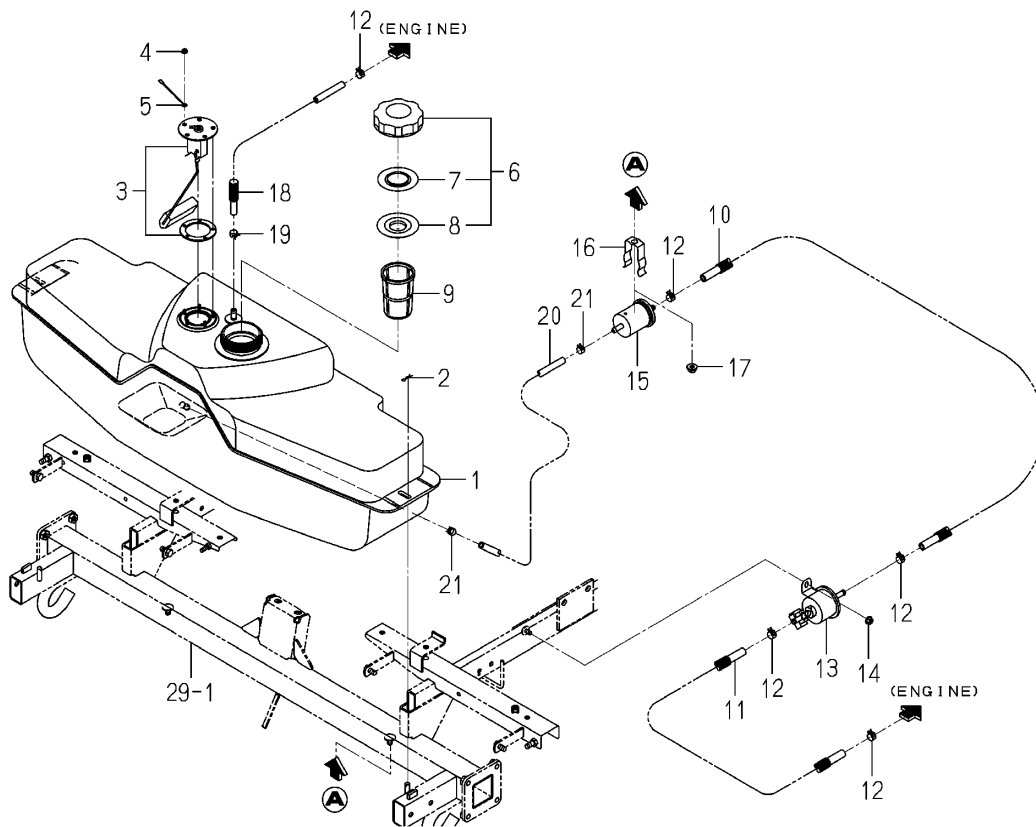
Fig.005 Tank(Fuel)system
