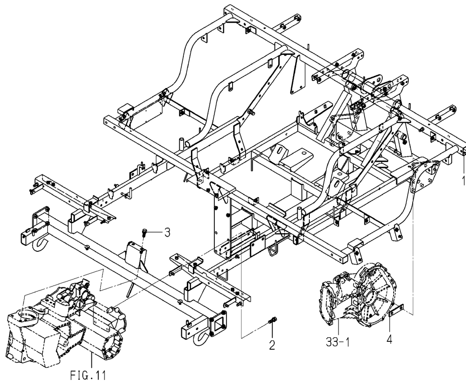
Fig.029 Frame(Main)system
