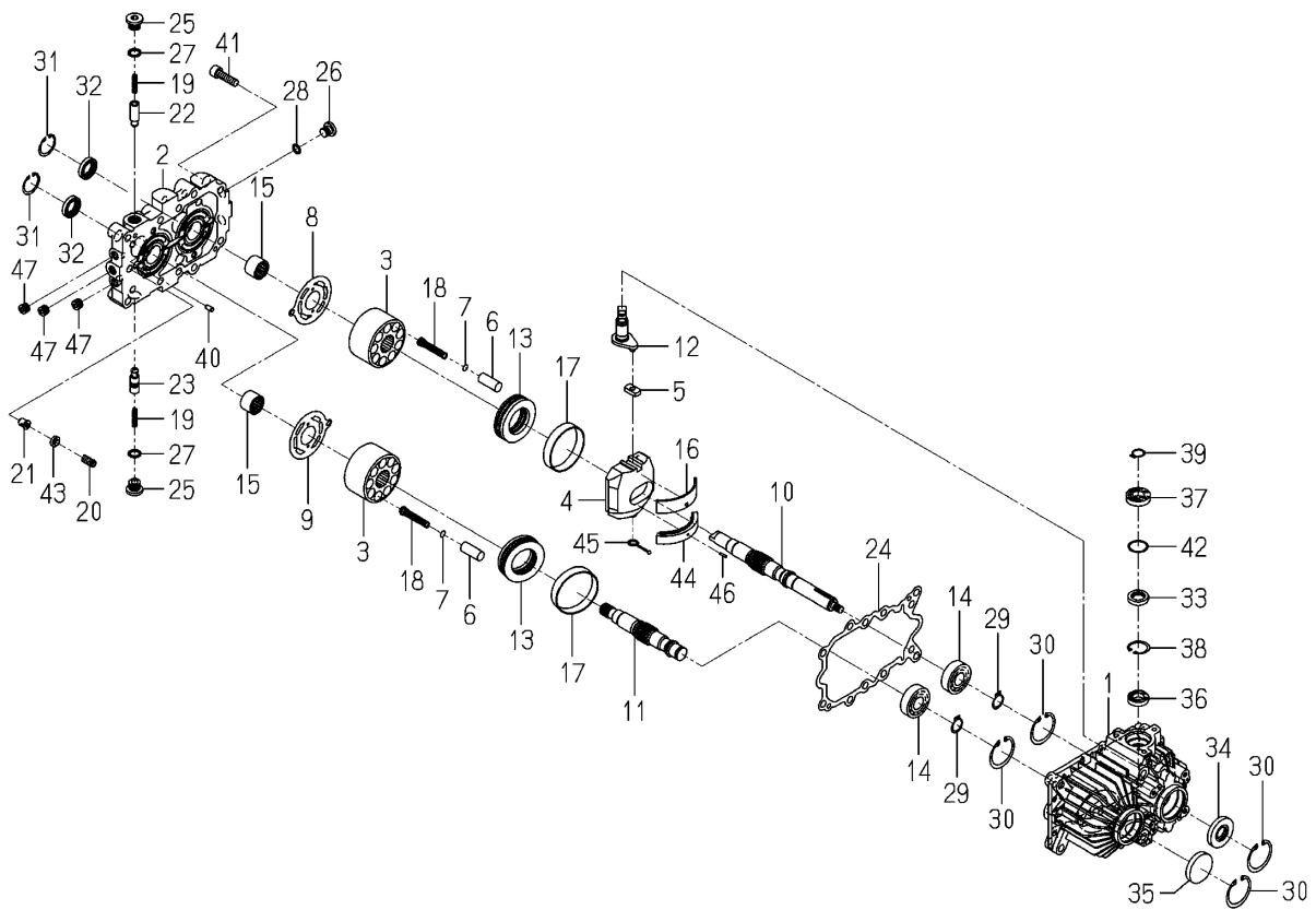
Fig.130 Component Partsfor K510-029-000-10 On Fig.87
