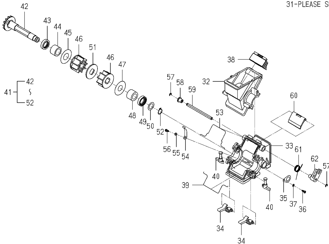
Fig.094a Send Out(Fertilizer)system(2/3)
