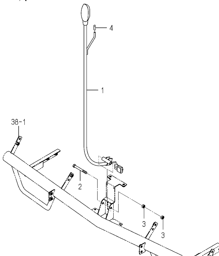
Fig.061 Marker(Center)system
