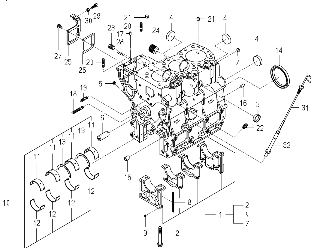
Fig.005 Cylinder Block
