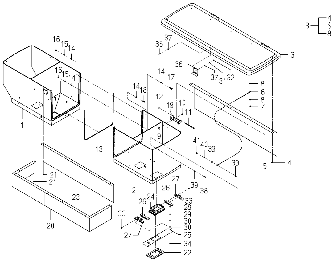
Fig.135 Component Partsfor 2233-688-320-20 On Fig.95
