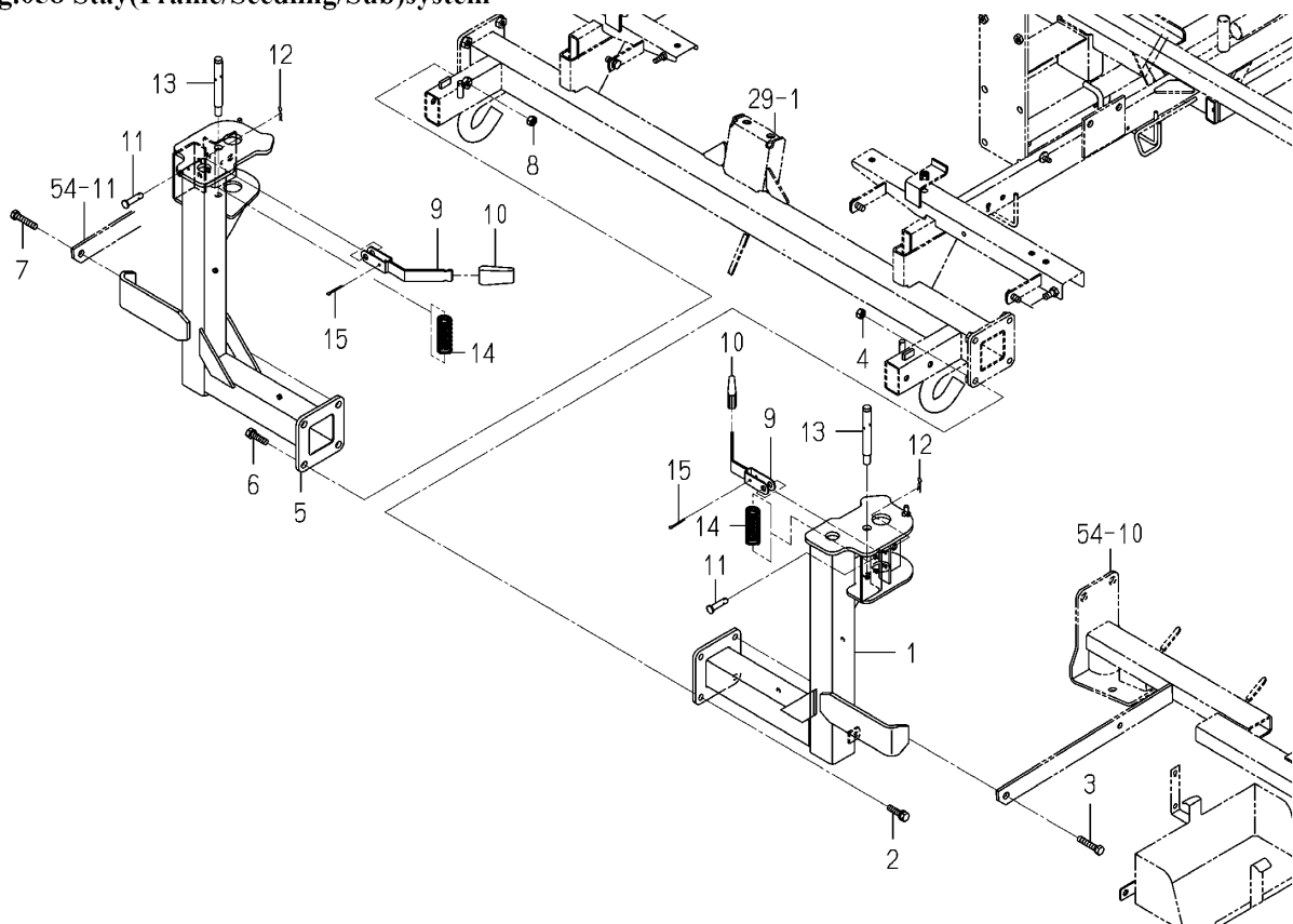
Fig.058 Stay(Frame/Seedling/Sub)system
