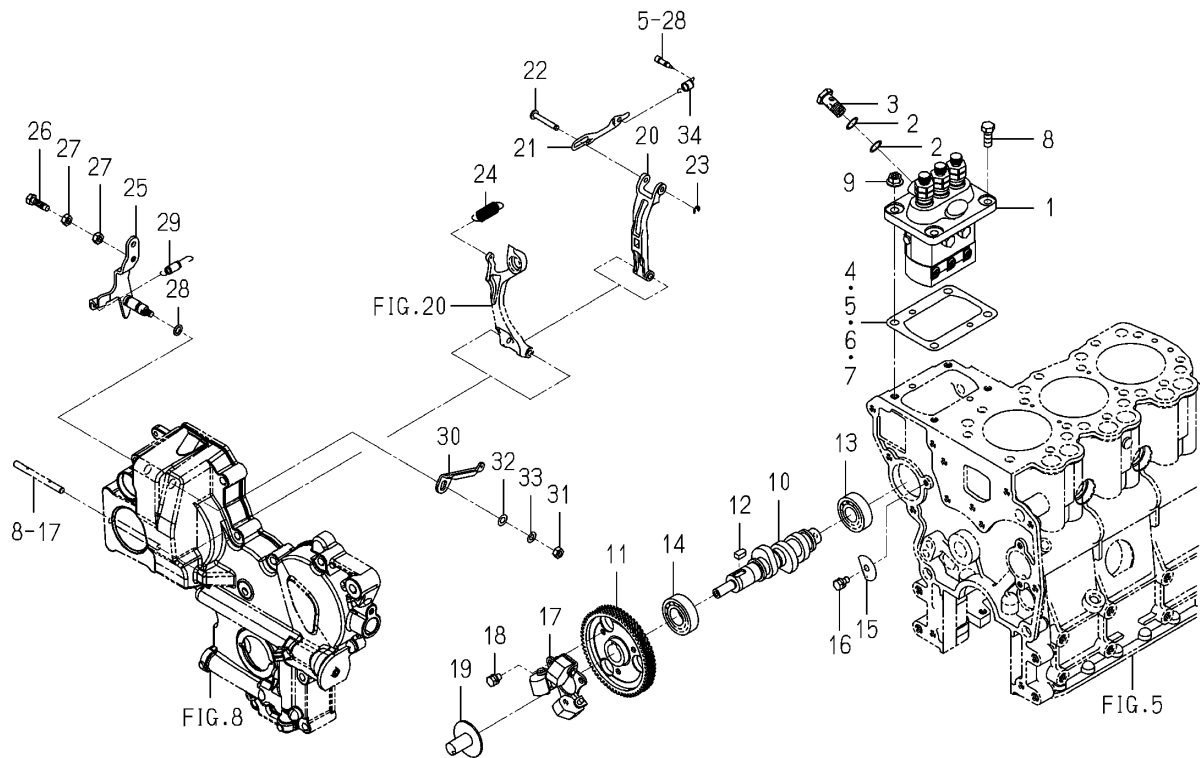
Fig.018 Injection Pump
