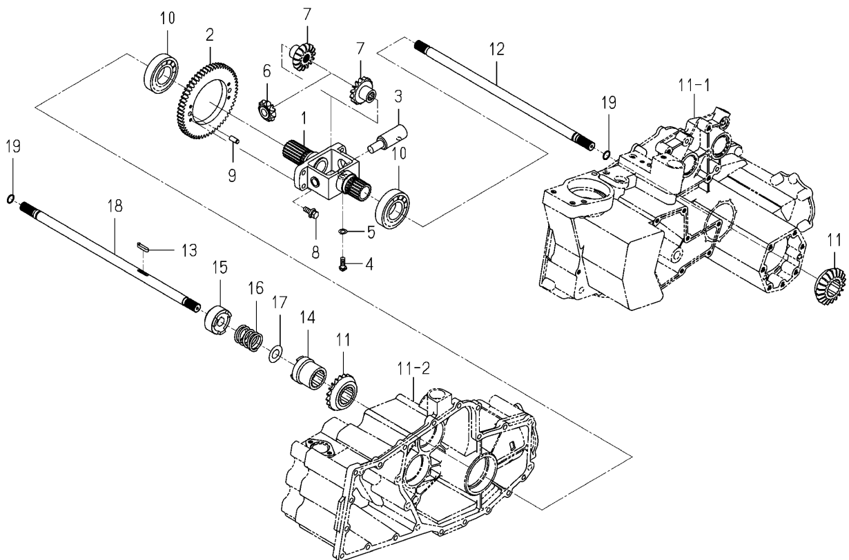
Fig.016 Shaft(Drive/Front)system
