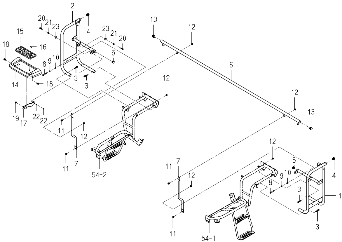
Fig.060 Handrail System
