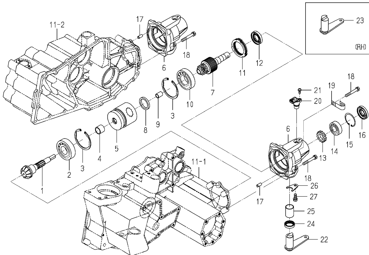
Fig.015 Shaft(Rear),clutch&brake System
