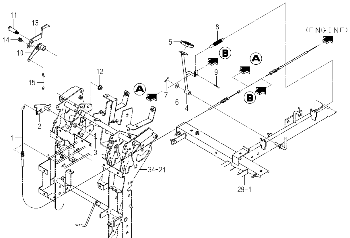
Fig.010 Pedal(Accelerator)system
