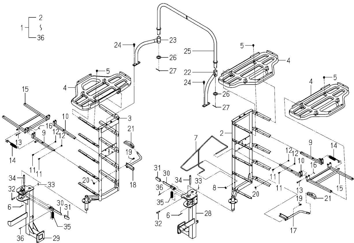
Fig.122 Seedling(Frame)set(Option)
