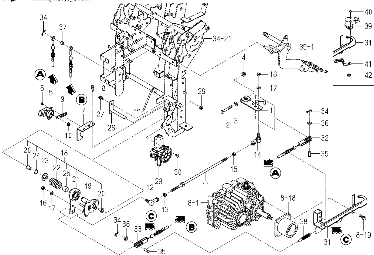
Fig.009 Link(Hst)system
