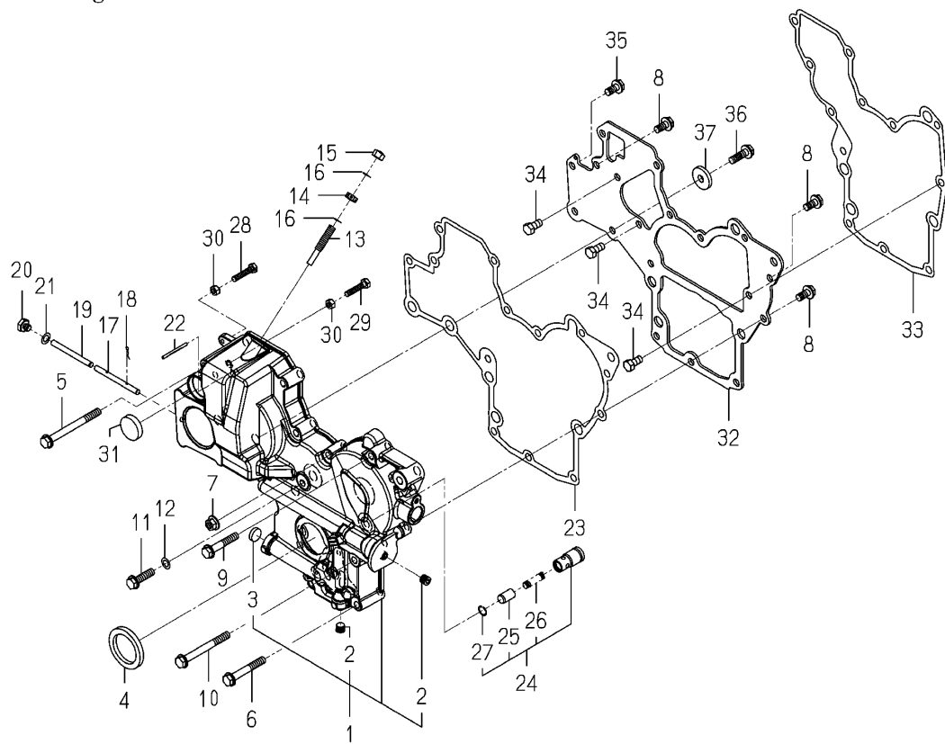
Fig.008 Timing Gear Case
