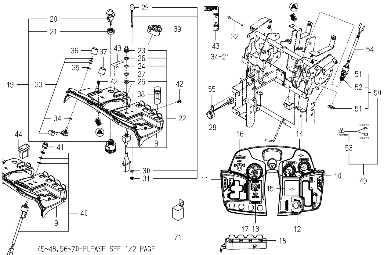
Fig.065a Panel(Instrument)system(2/2)
