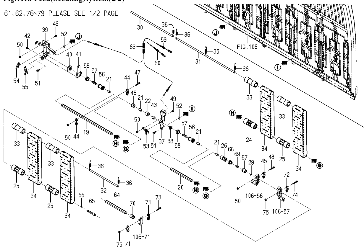
Fig.111a Feed(Seedling)system(2/2)
