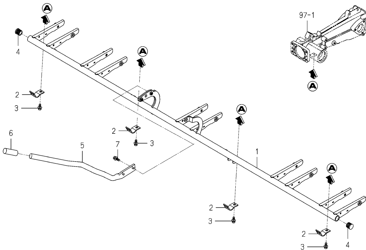
Fig.084 Lever(Depth/Planting)system
