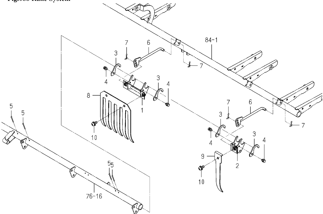
Fig.088 Rake System
