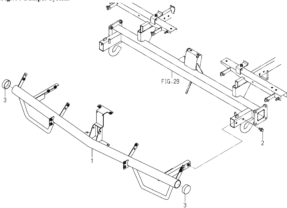
Fig.038 Bumper System
