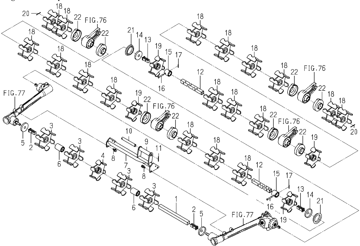
Fig.075 Rotor System
