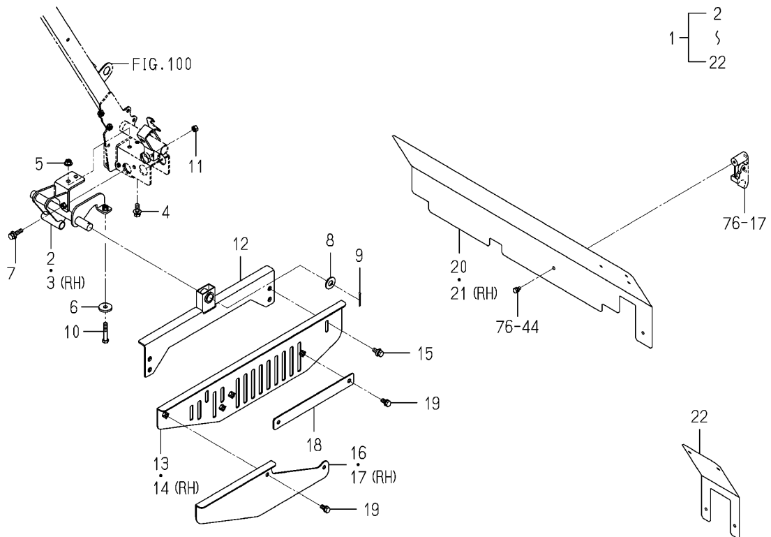
Fig.125 Guard Plate Set(Optional)
