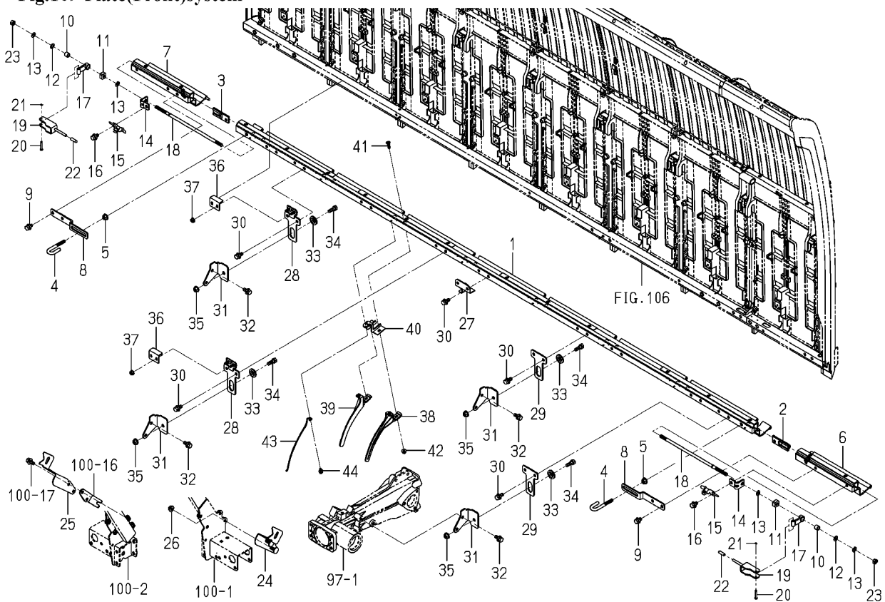
Fig.109 Plate(Front)system
