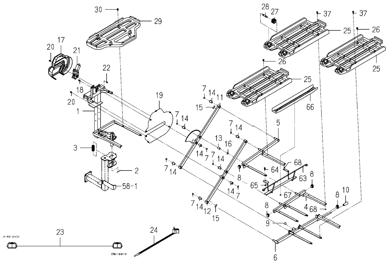
Fig.056 Tray(Seedling/Sub)system(1/2)
