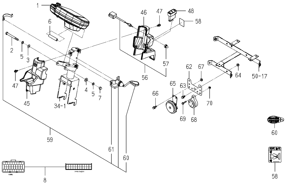
Fig.065 Panel(Instrument)system(1/2)
