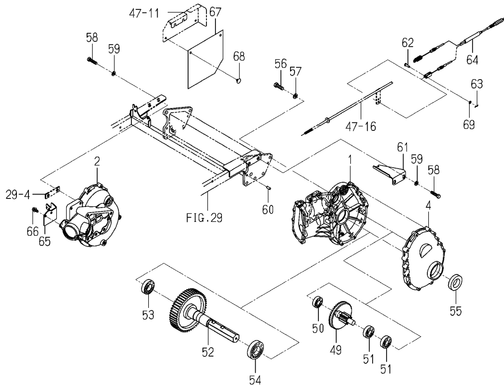
Fig.033a Case(Rear)system(2/2)
