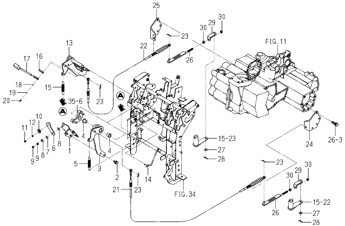
Fig.036 Pedal(Brake)system
