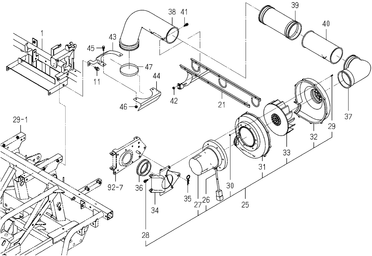
Fig.093a Frame(Fertilizer)system(2/2)
