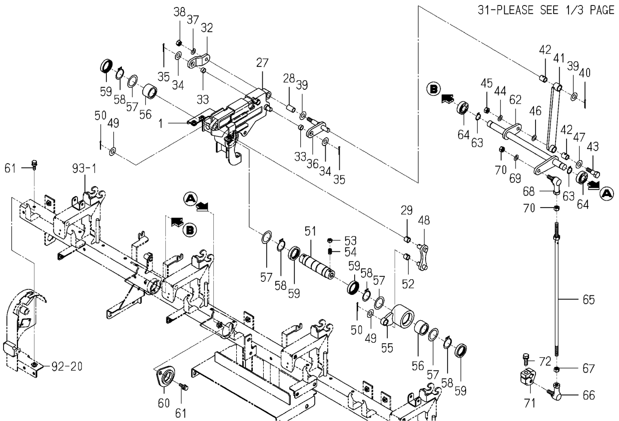
Fig.089a Drive(Fertilizer)system(2/3)
