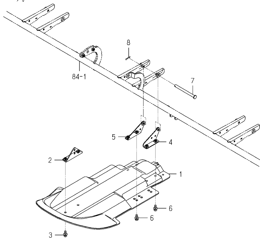
Fig.085 Float(Center)system
