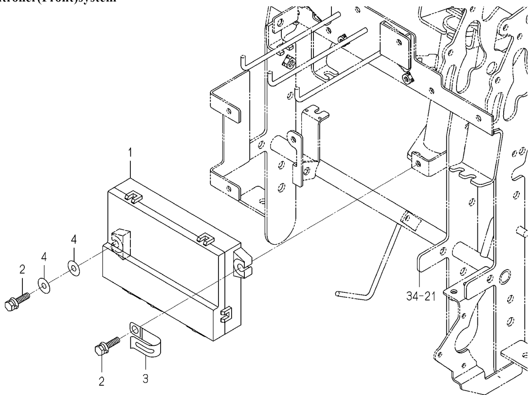
Fig.069 Controller(Front)system
