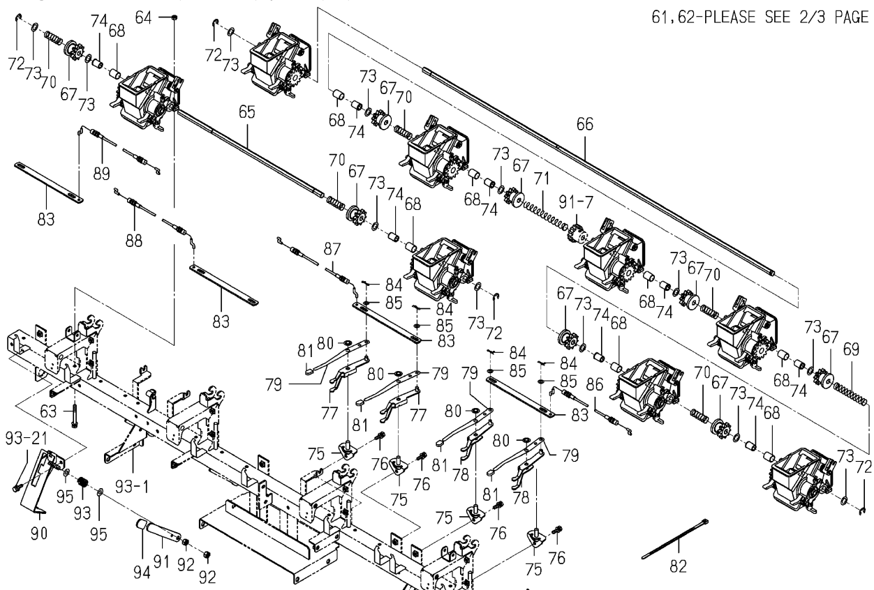
Fig.094b Send Out(Fertilizer)system(3/3)
