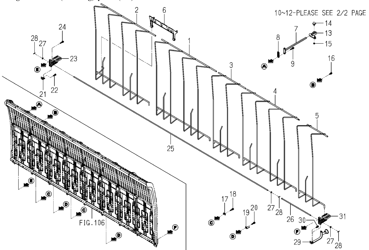
Fig.110 Holder(Seedling)system(1/2)
