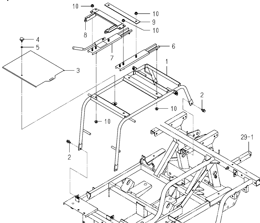
Fig.055 Seat System
