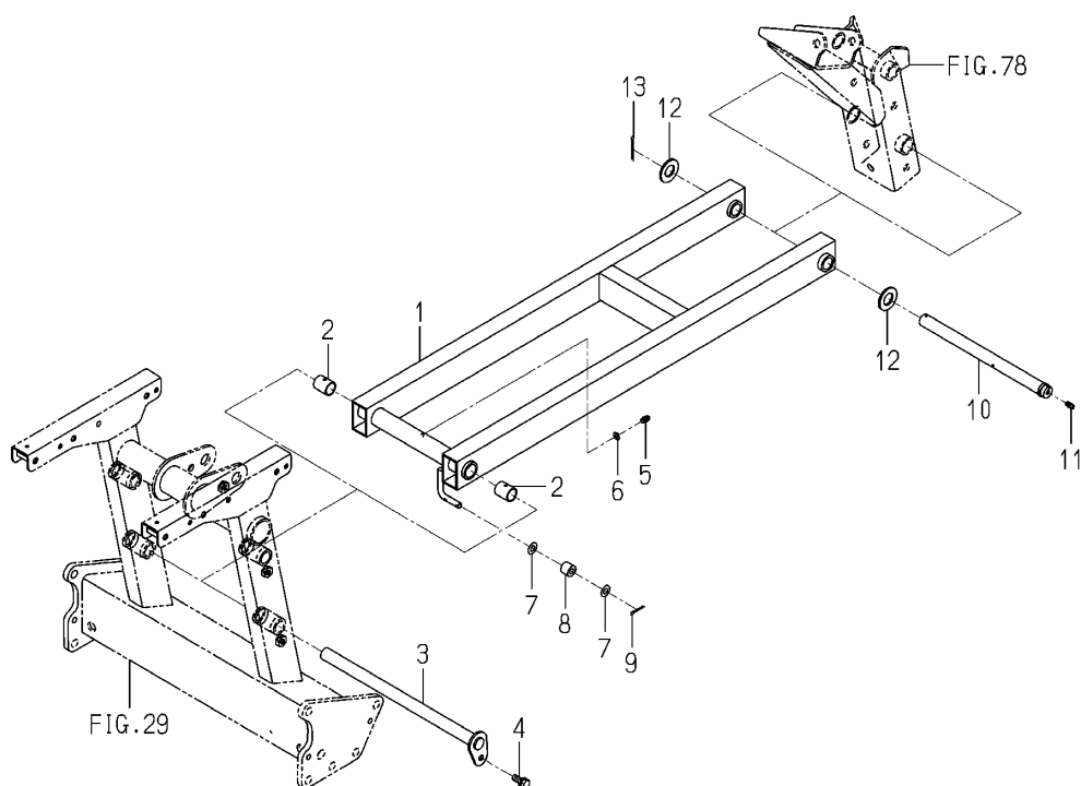
Fig.045 Link(Lower)system
