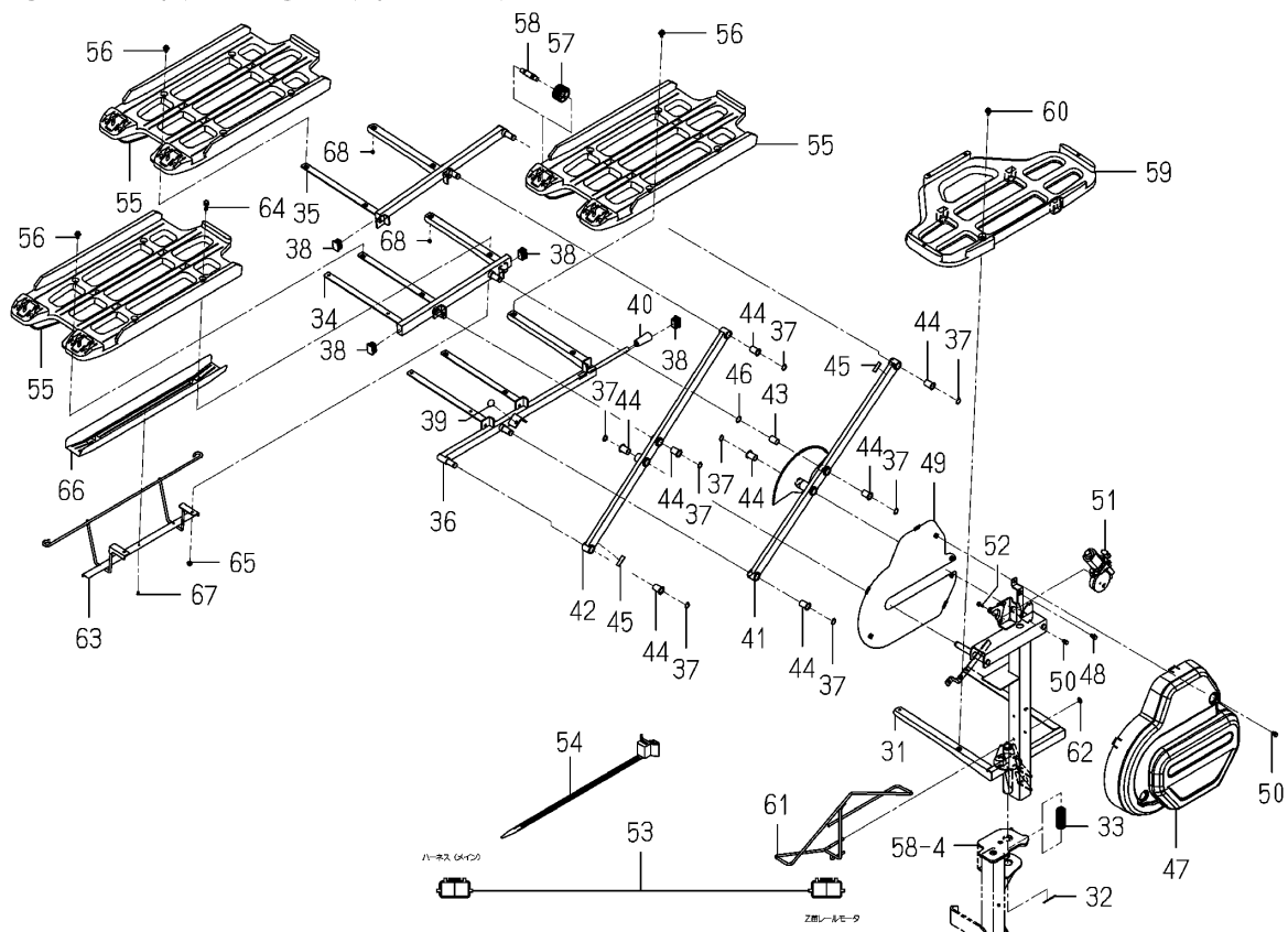
Fig.056a Tray(Seedling/Sub)system(2/2)
