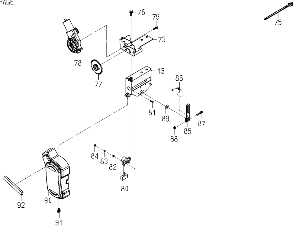
Fig.089b Drive(Fertilizer)system(3/3)
