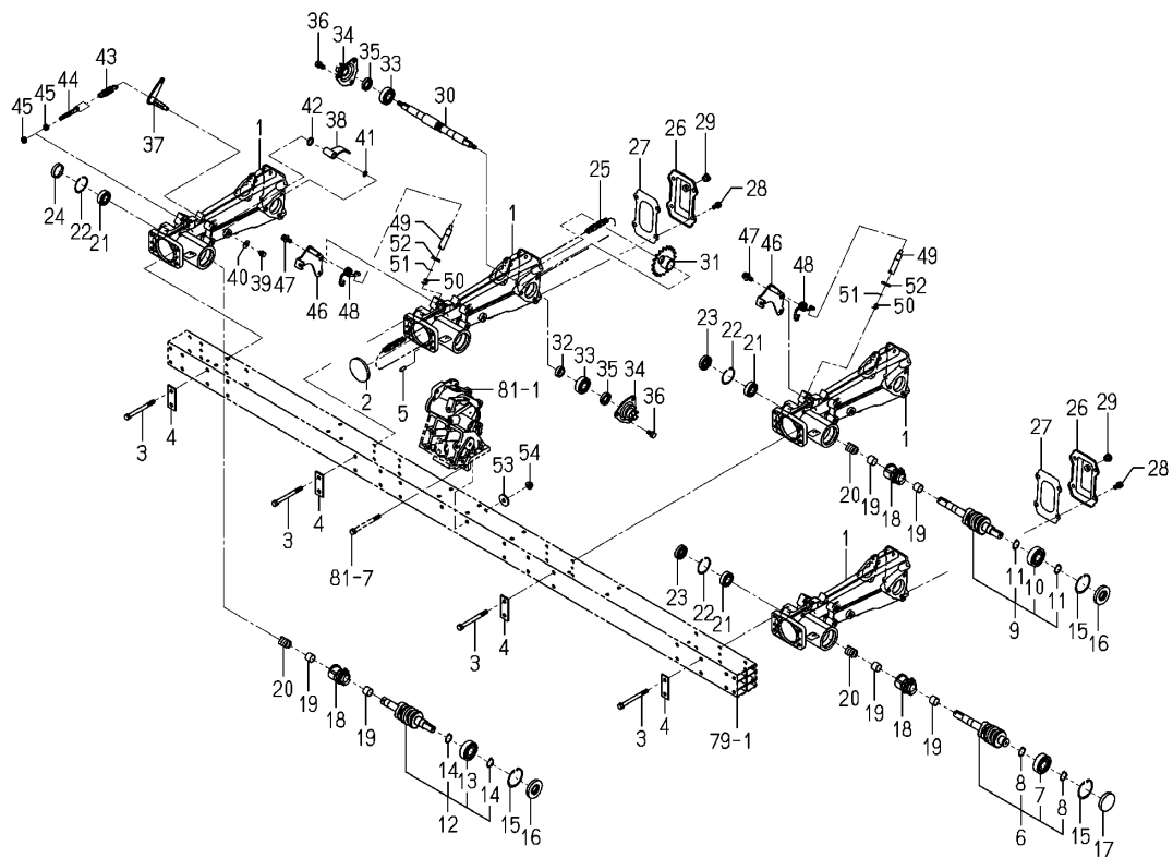
Fig.097 Frame(Side)system
