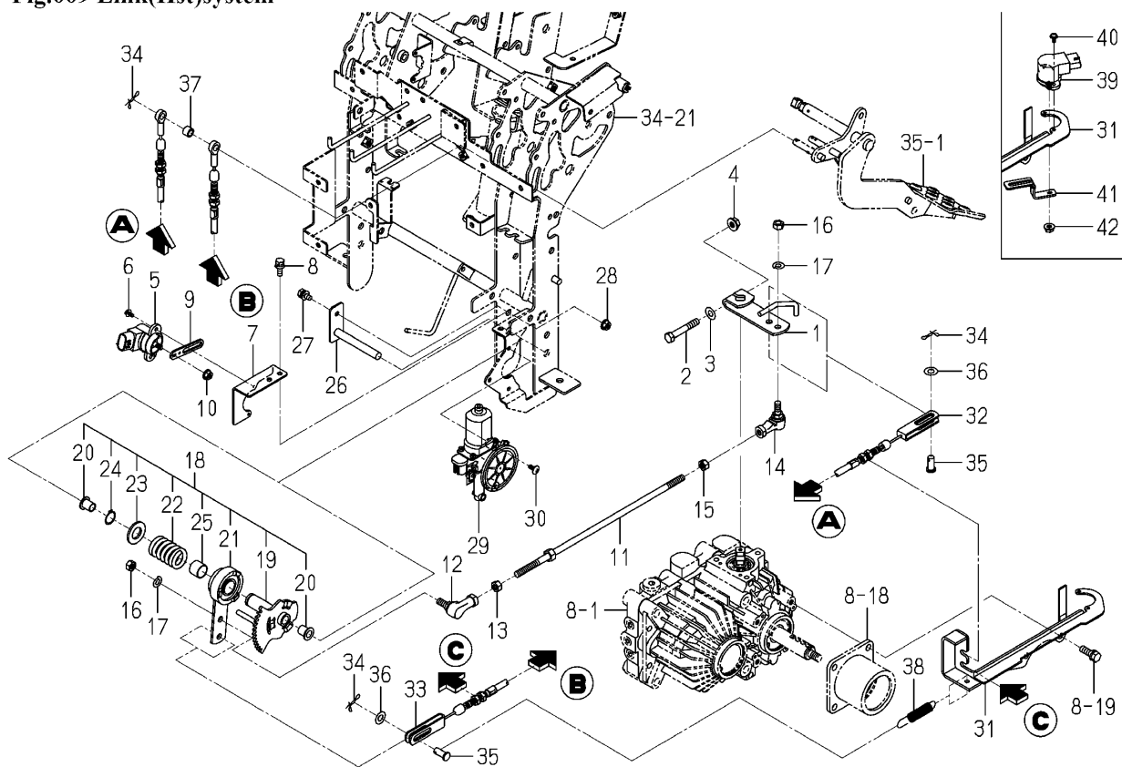
Fig.009 Link(Hst)system
