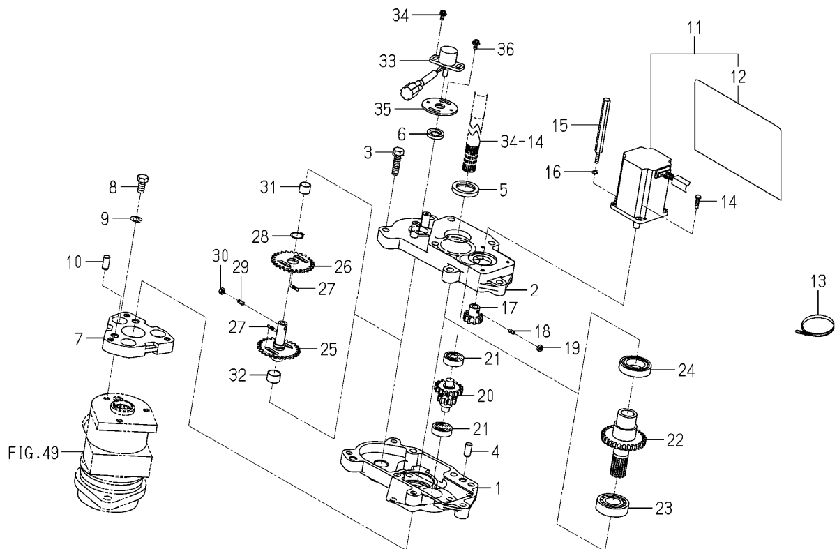
Fig.039 Motor(Unit/Drive)system
