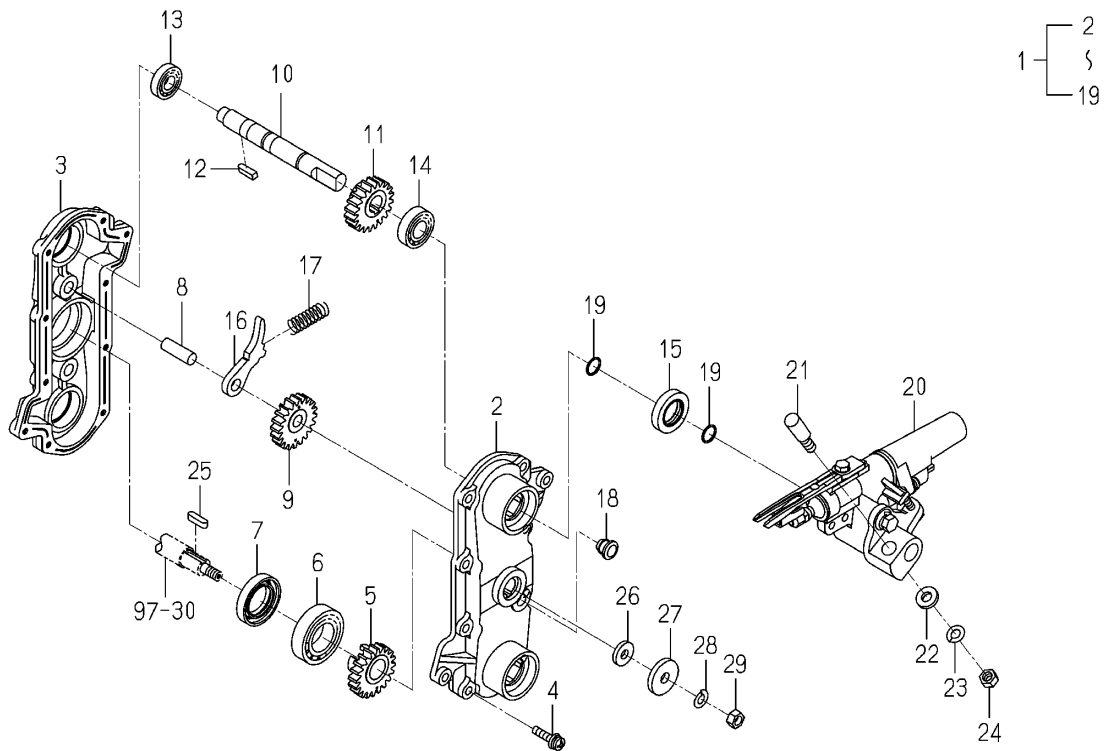
Fig.104 Planter(Lh)system
