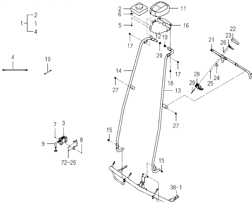
Fig.071 Sensor(Gnss)setsystem
