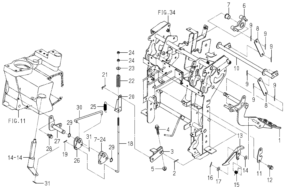
Fig.035 Pedal(Brake/Parking)system
