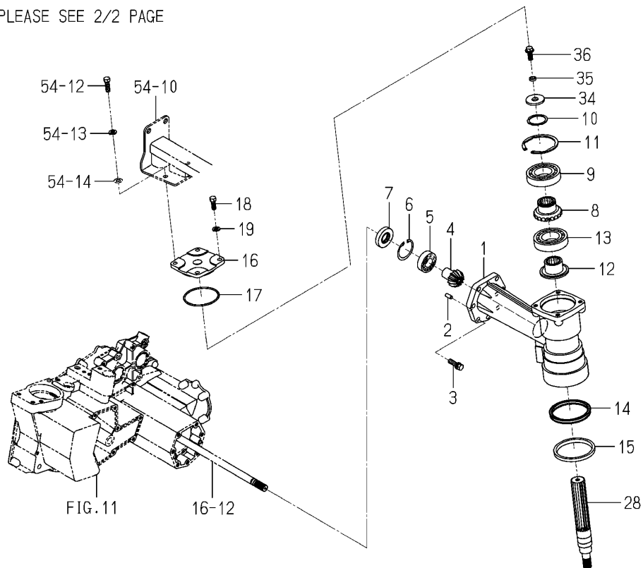
Fig.026 Case(Gear/Final)system(1/2)
