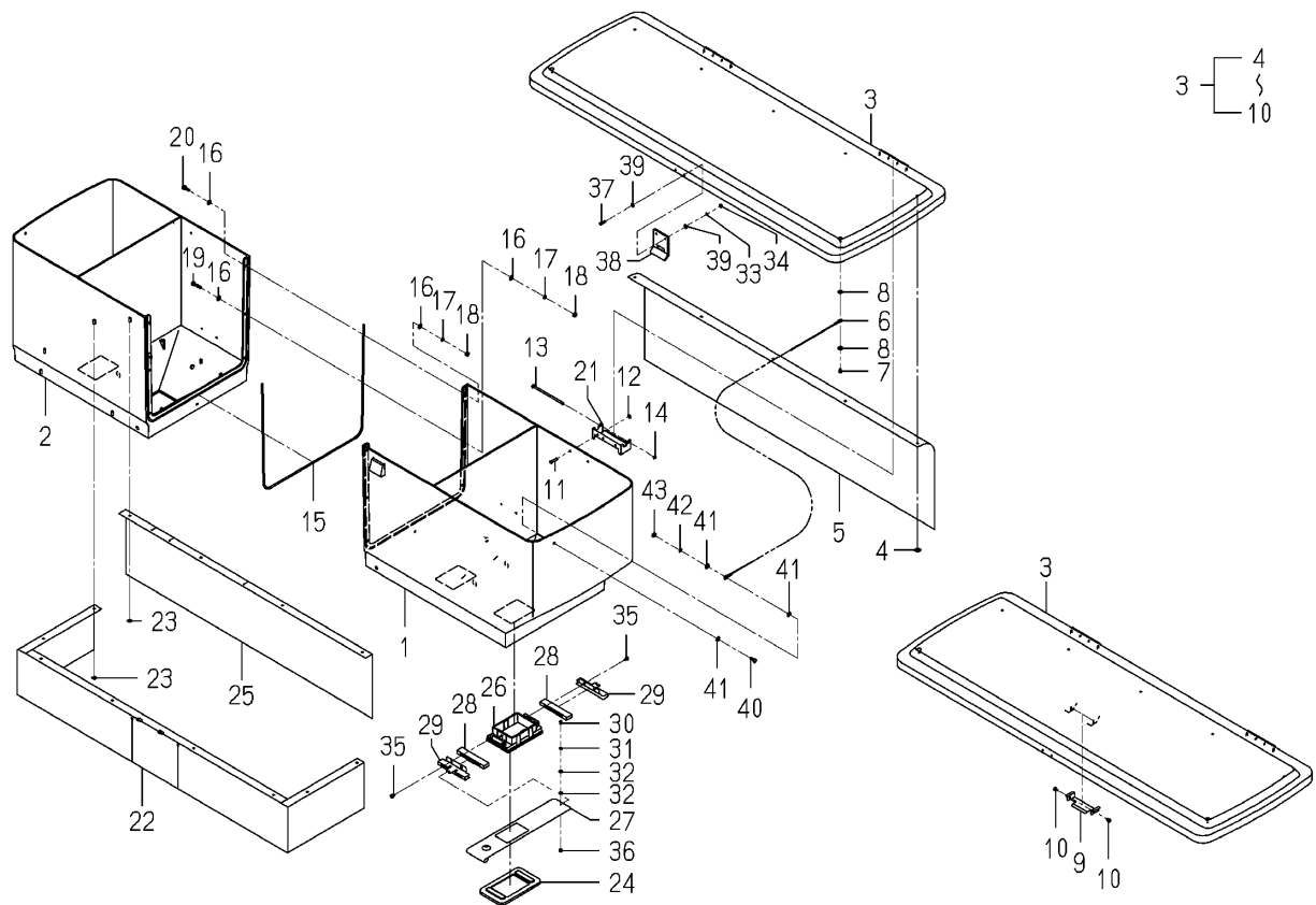
Fig.134 Component Partsfor 2233-688-310-20 On Fig.95
