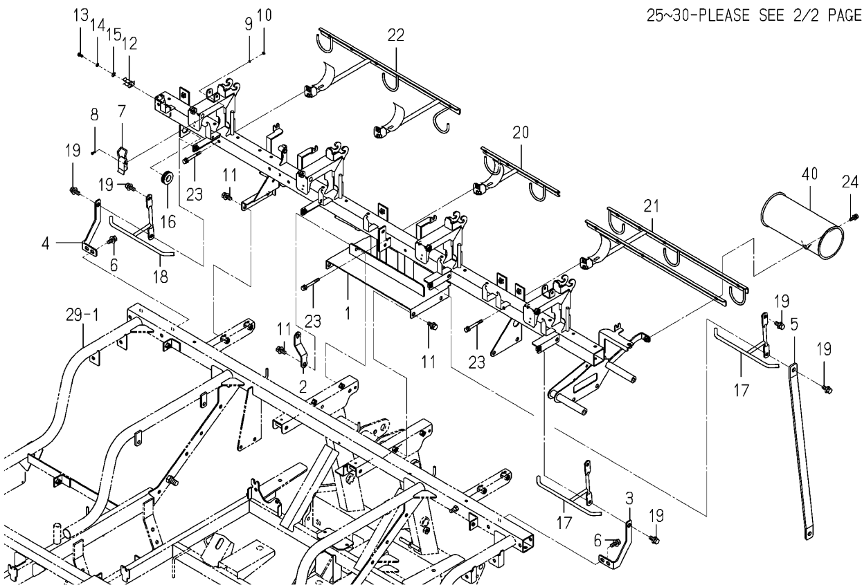
Fig.093 Frame(Fertilizer)system(1/2)
