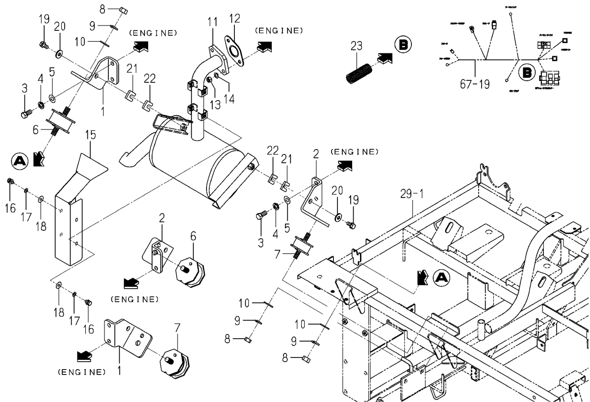
Fig.001 Bracket(Engine)&amp;muffler System
