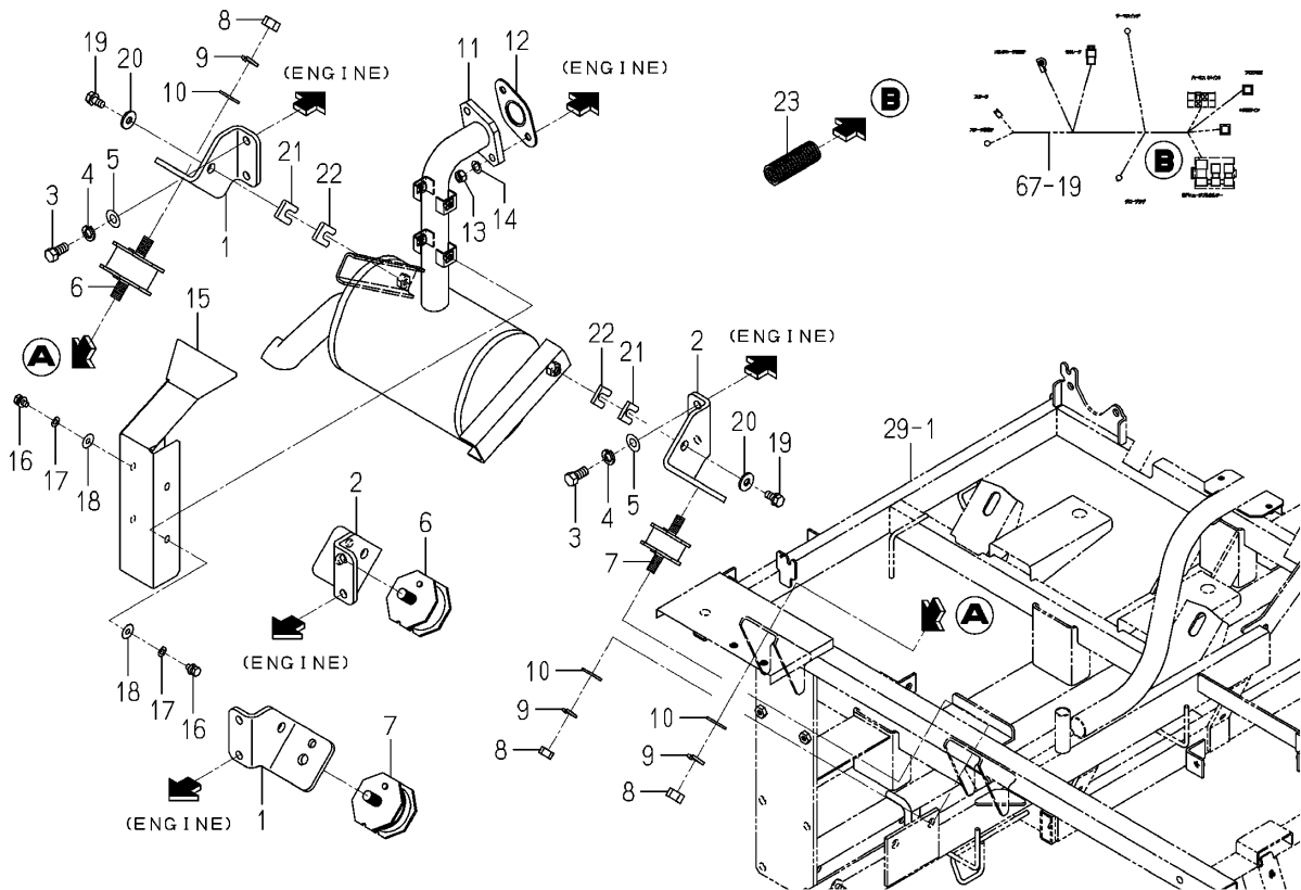
Fig.001 Bracket(Engine)&muffler System
