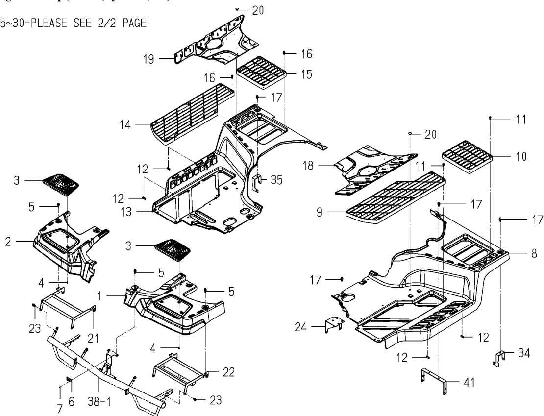
Fig.052 Step(Front)system(1/2)
