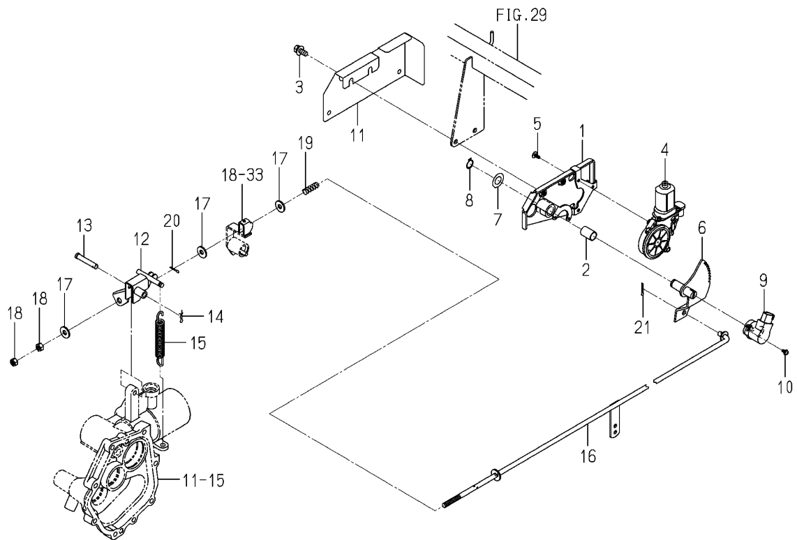
Fig.047 Clutch(Planting)system
