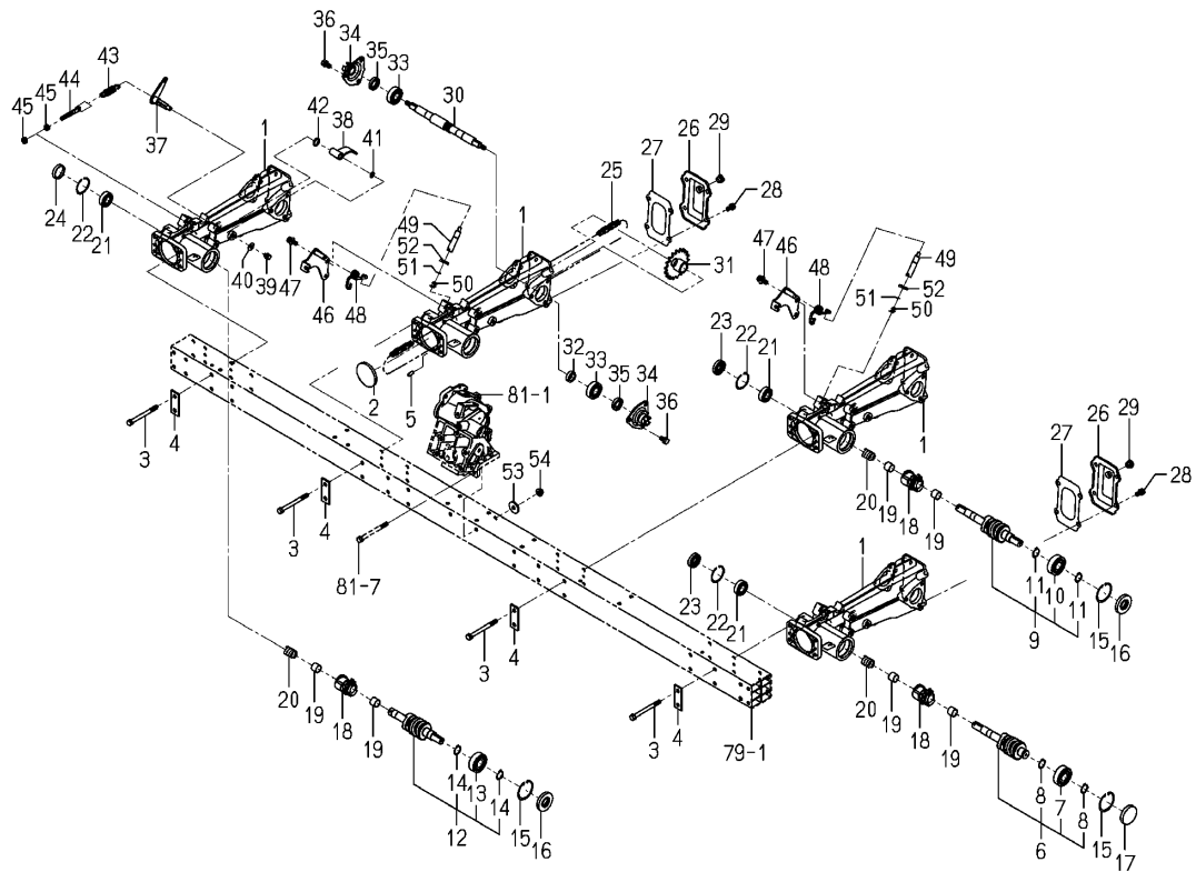
Fig.097 Frame(Side)system
