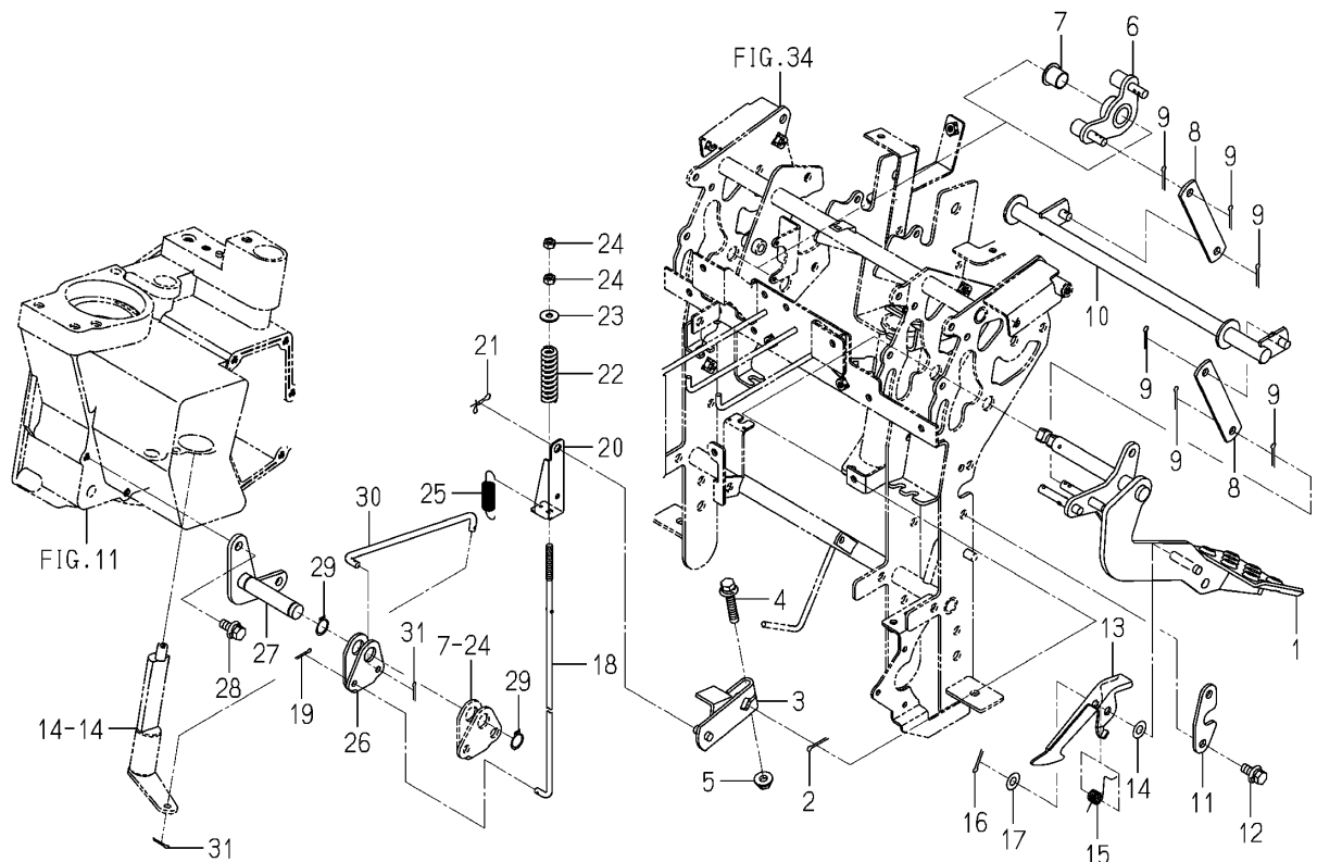
Fig.035 Pedal(Brake/Parking)system
