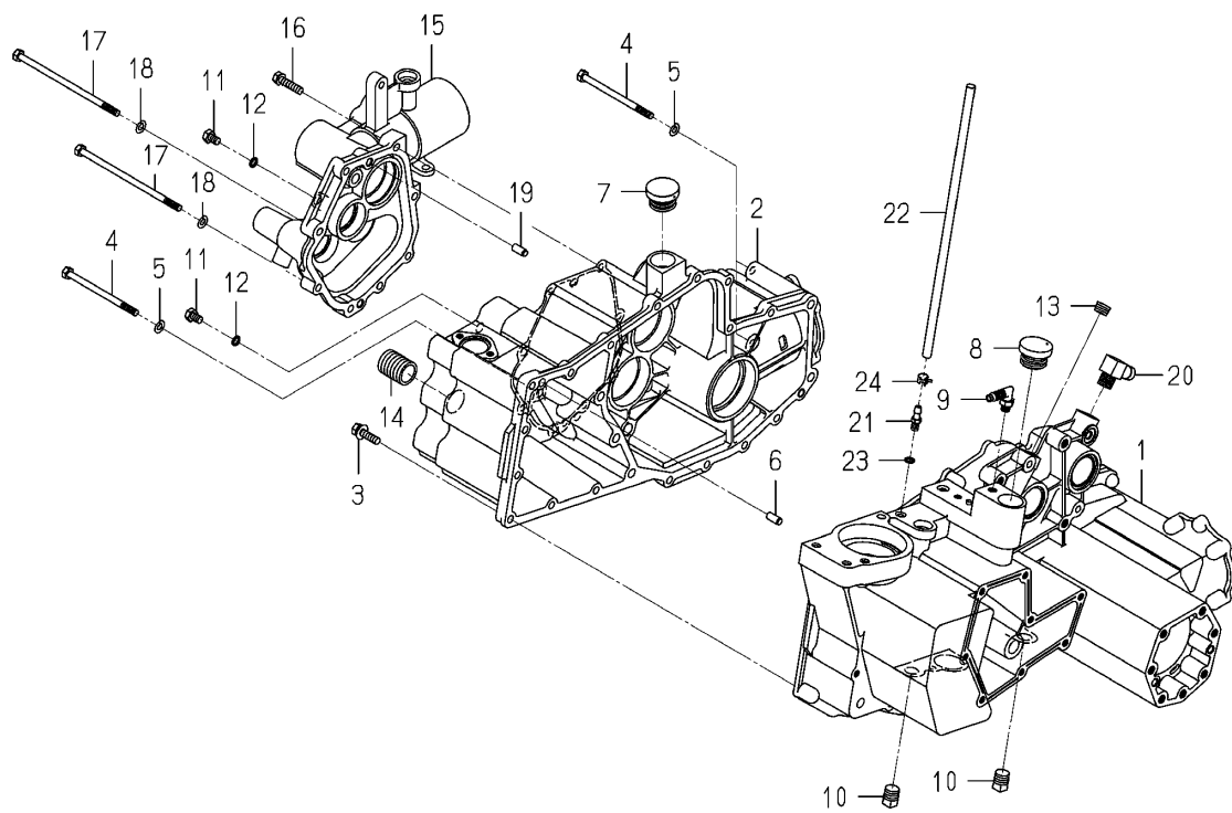
Fig.011 Case(Transmission)system
