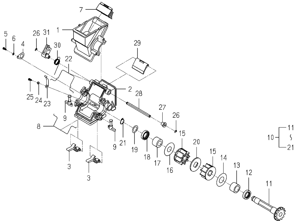
Fig.094 Send Out(Fertilizer)system(1/3)
