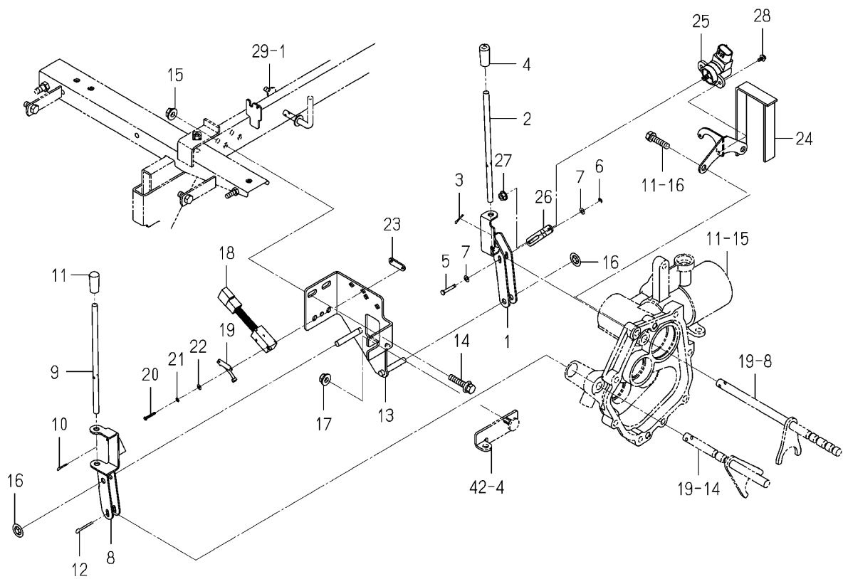
Fig.020 Lever(Planting Interval)system
