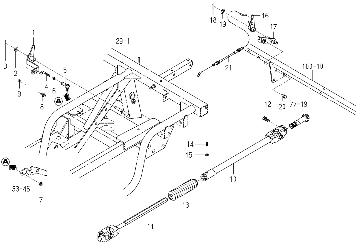
Fig.074 Drive(Rotor)system
