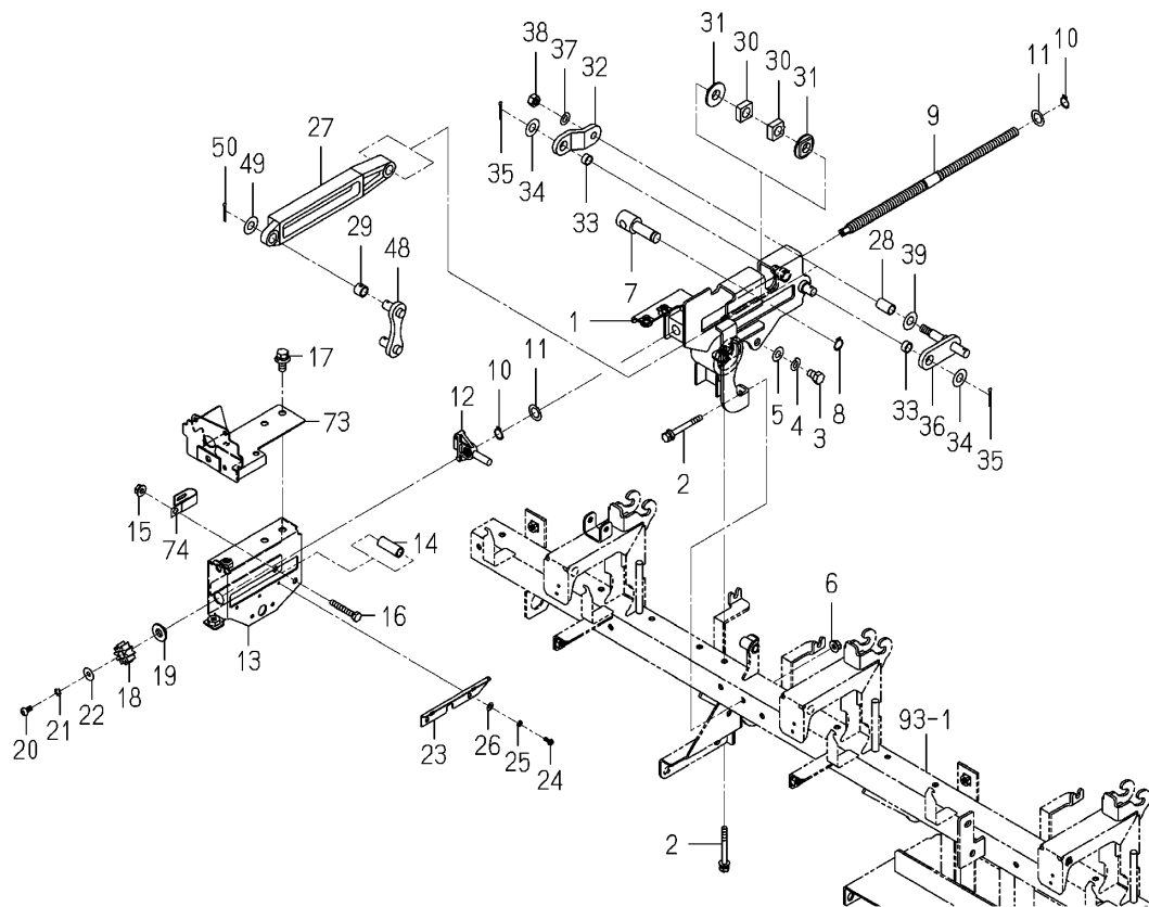
Fig.089 Drive(Fertilizer)system(1/3)
