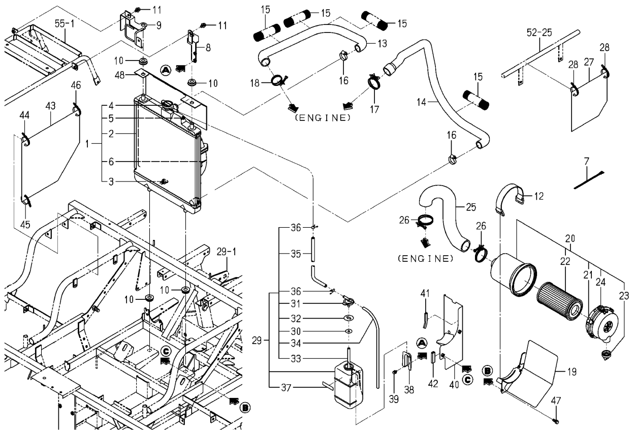
Fig.002 Radiator&cleaner(Air)system
