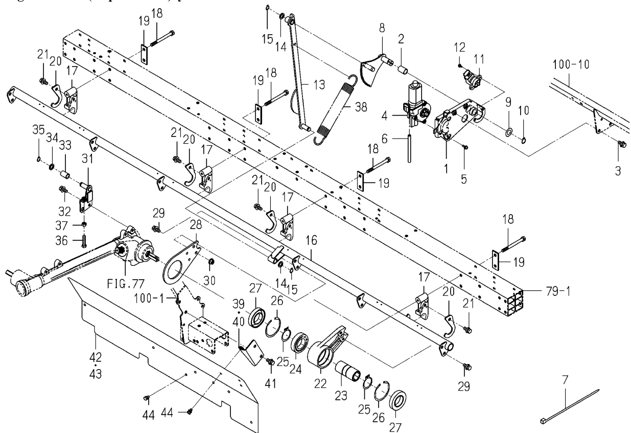
Fig.076 Lever(Depth/Rotor)system
