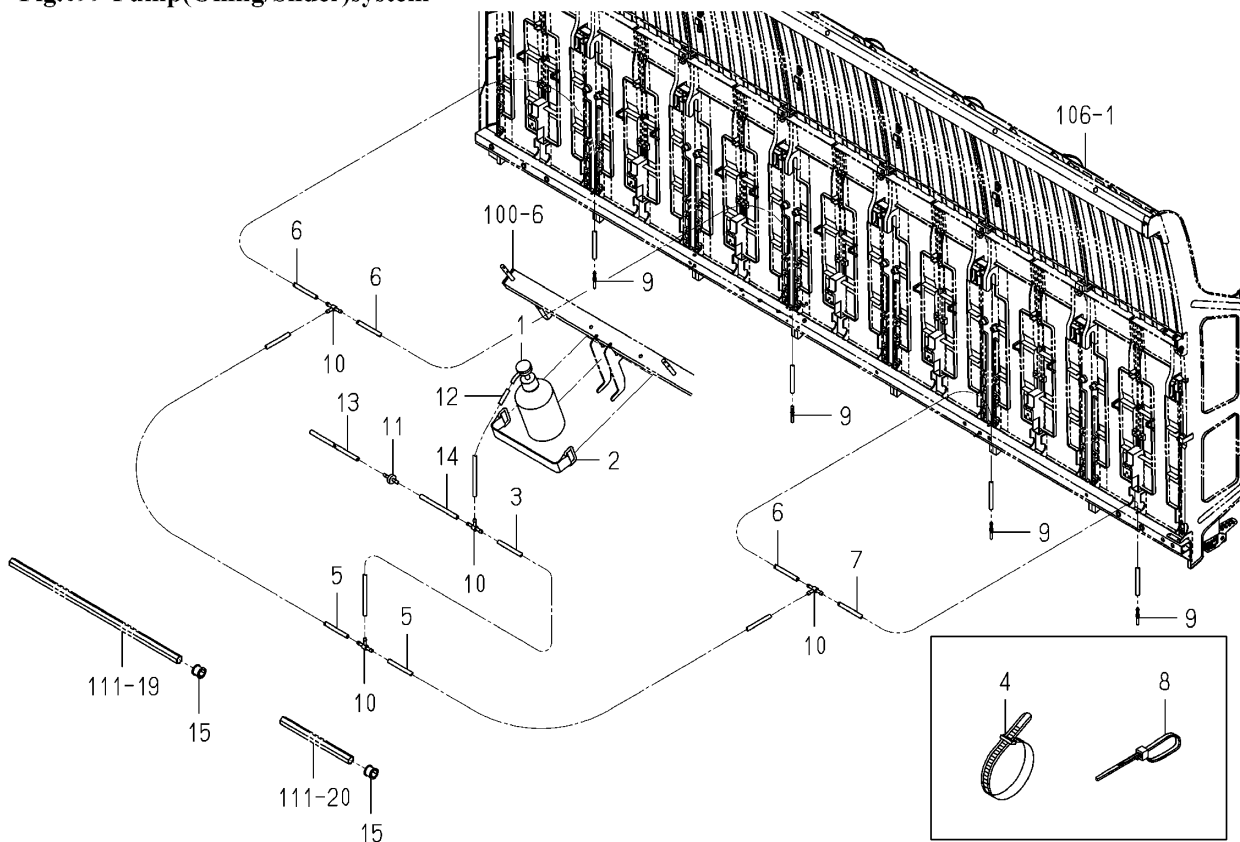
Fig.099 Pump(Oiling/Slider)system
