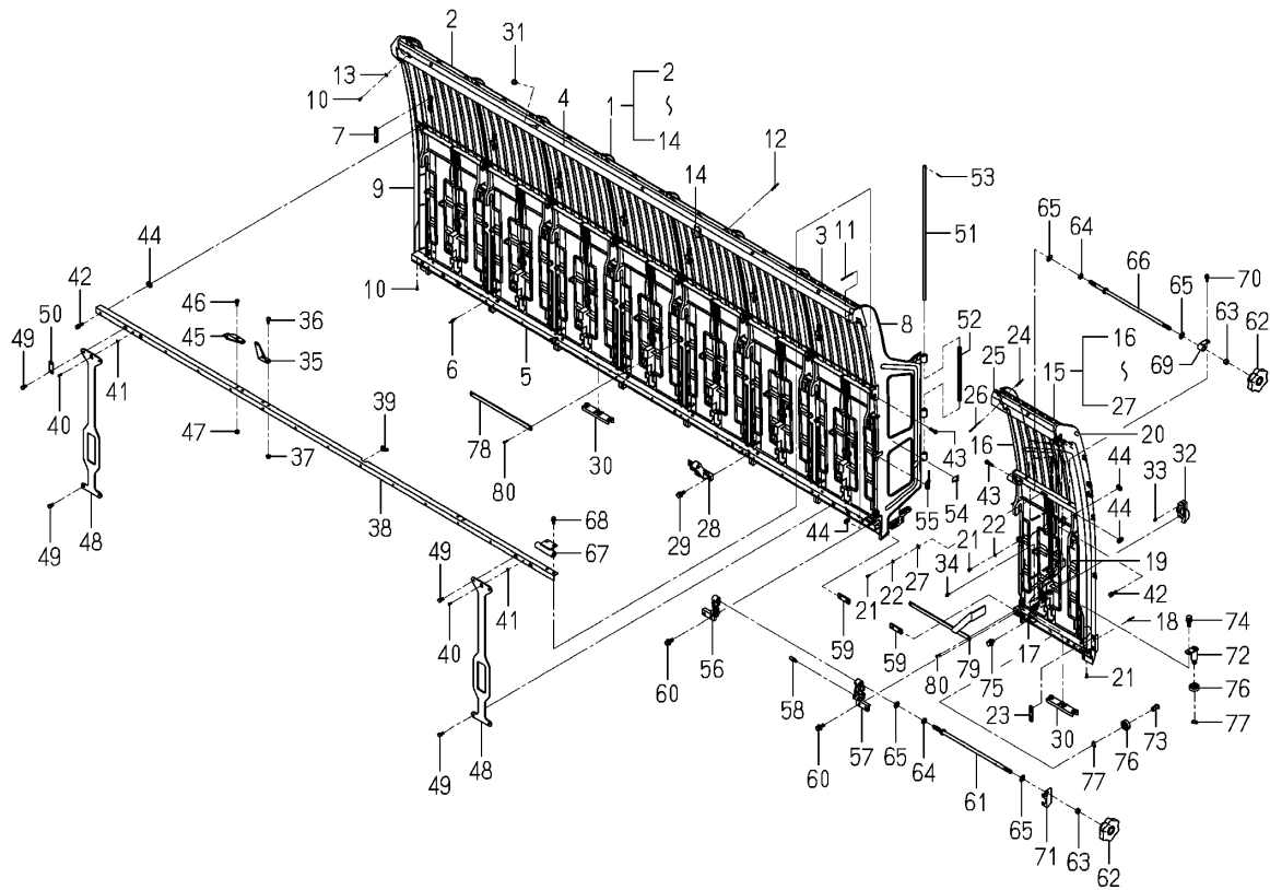
Fig.106 Tank(Seedling)system
