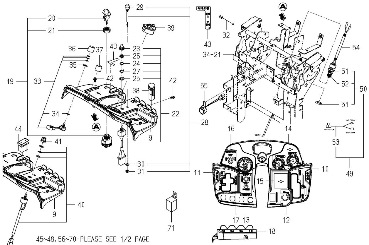
Fig.065a Panel(Instrument)system(2/2)
