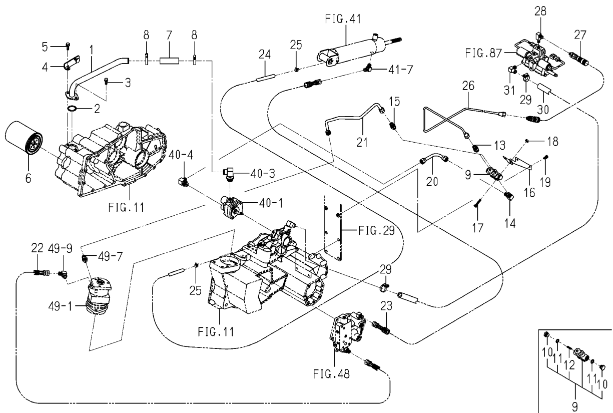
Fig.042 Piping System(1/2)
