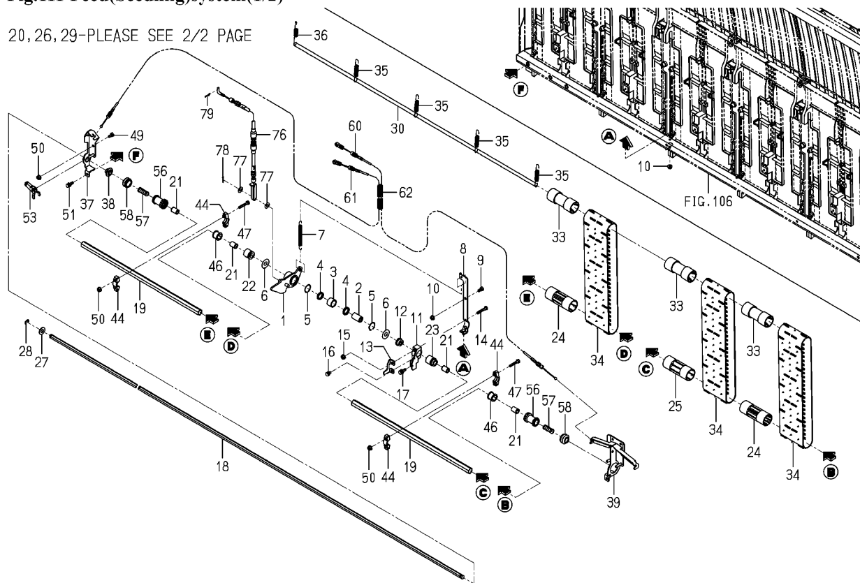
Fig.111 Feed(Seedling)system(1/2)
