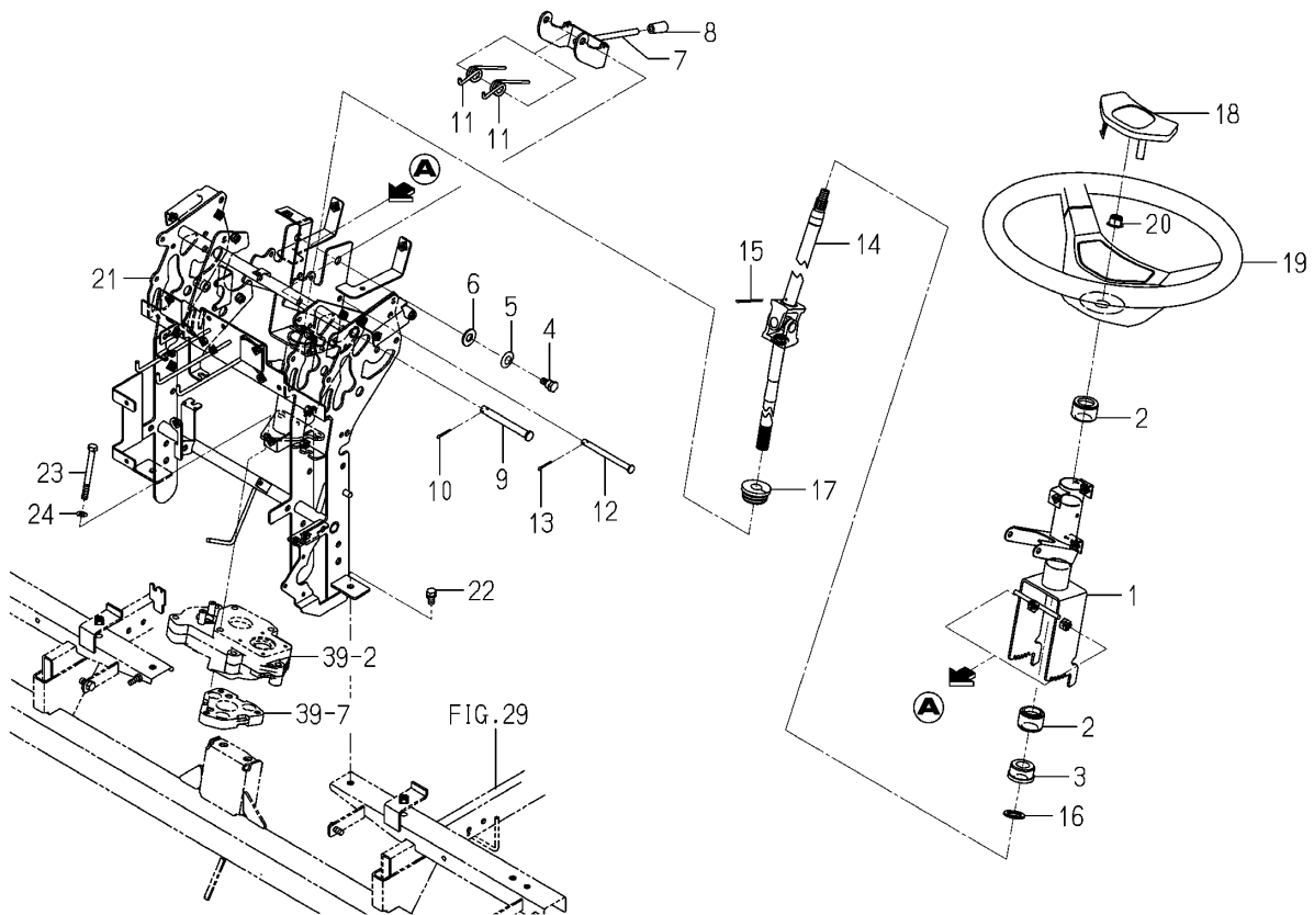
Fig.034 Wheel(Steering)system
